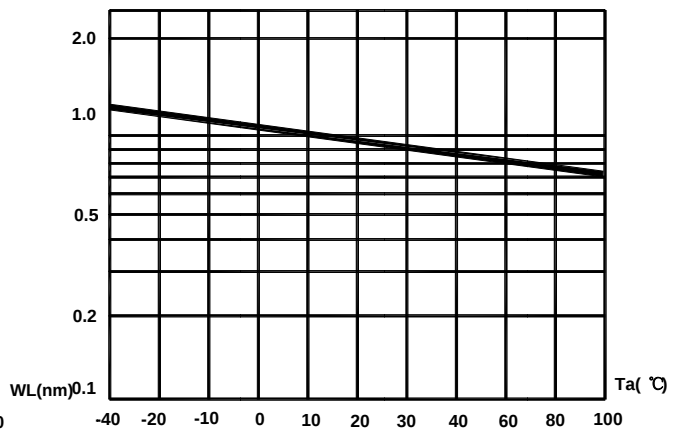
Relative Luminous Intensity vs. Ambient Temperature
